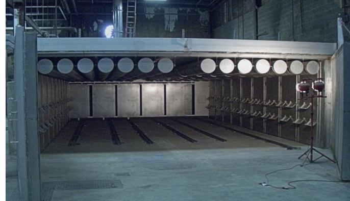
Curing oven fully installed at the customer's facility.
